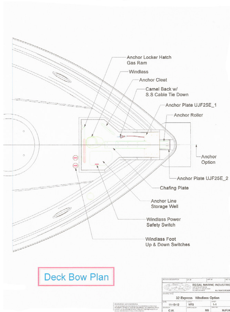
26 EXPRESS TYPICAL BOW PLAN-WINDLASS
